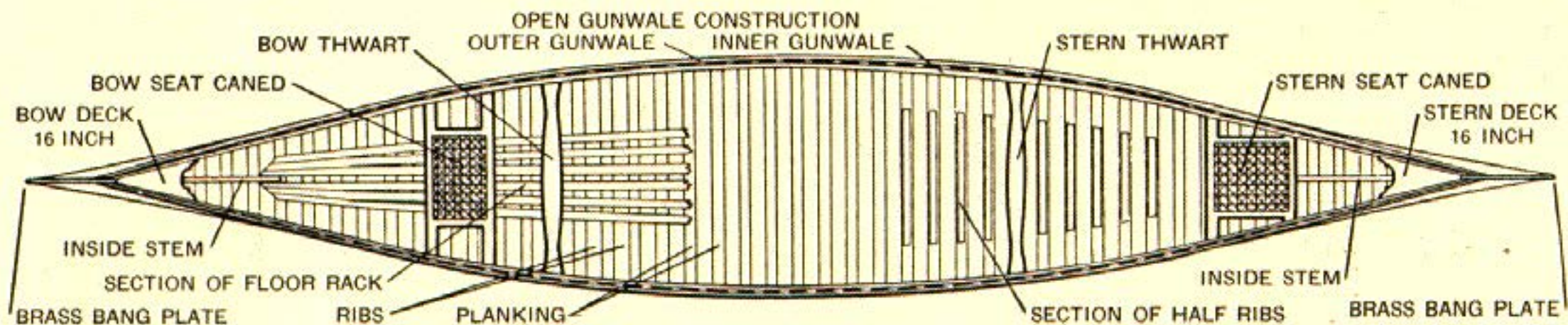
DIAGRAM of the "Old Town Canoe"
